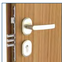
Main lock class 7 3-tumbler GERDA ZW 1000
