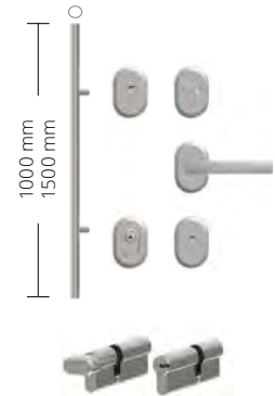
Montreal 1000 with A-A cylinders
